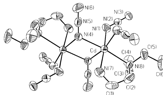
Fig. 5 Dimeric subunit of complex 4 with the atom numbering scheme.
